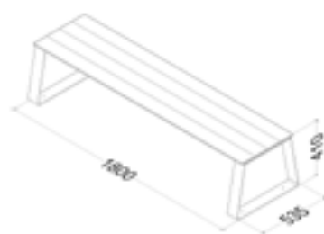
Banquette ref 30662
