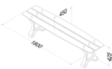
Banquette ref 31022
